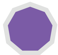
Nonagon
