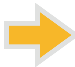
Arrow
